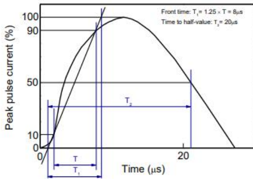
8/20 \mu\text{s} waveform per IEC61000-4-5
